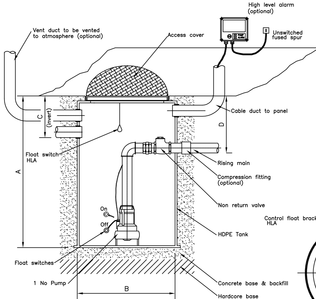
SIDE ELEVATION
